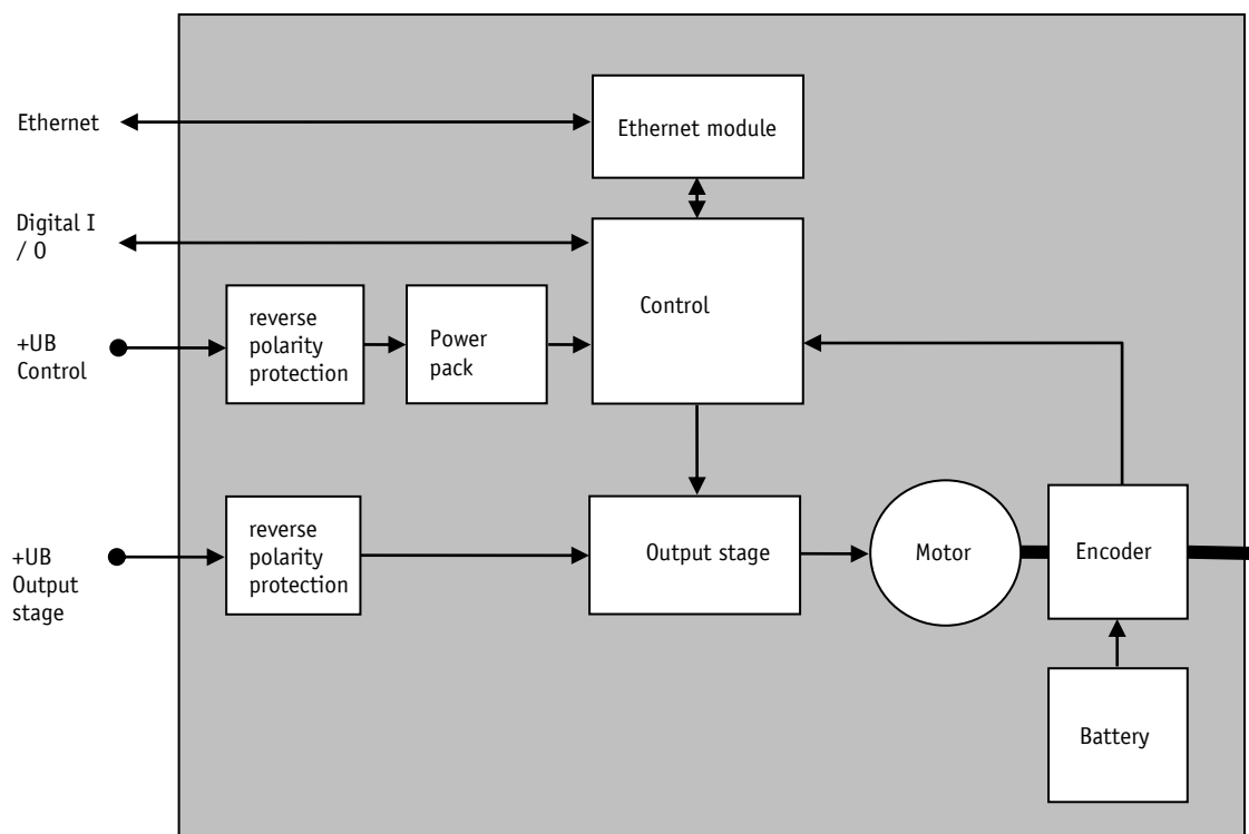
Fig. 18: Block diagram
