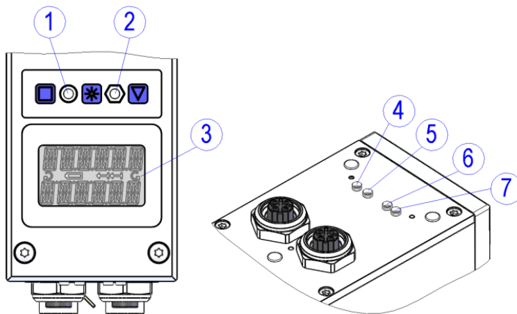
Fig. 1: Display and control elements
