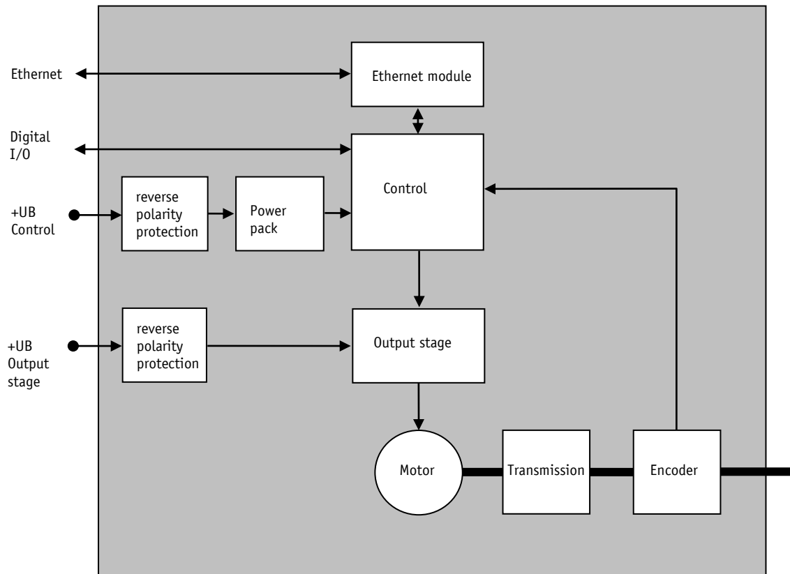
Fig. 22: Block diagram
