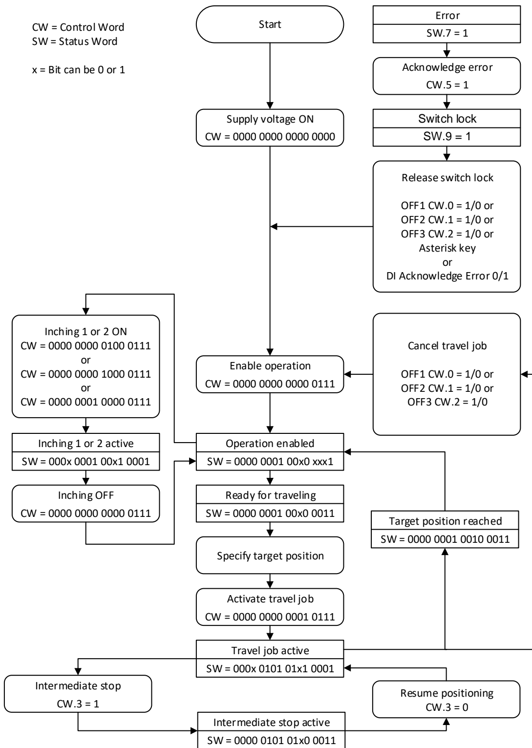
Fig. 9: Flowchart positioning mode
