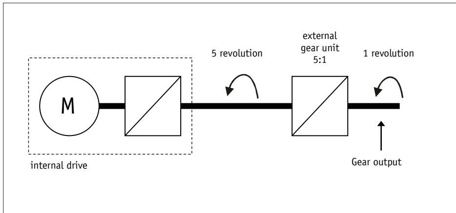
Fig. 3: External gear
