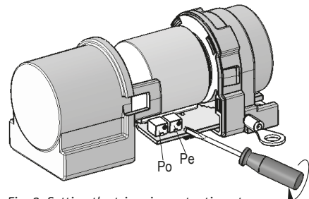
Fig. 8: Setting the trimming potentiometers
