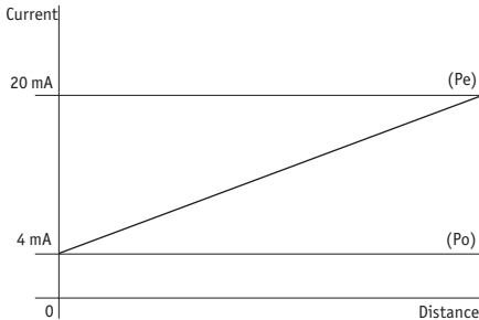
Fig. 9: Alignment
