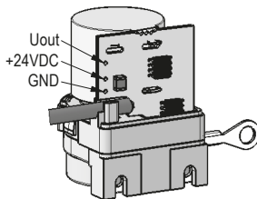
Fig. 7: Potentiometer connection MWU
