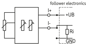
Fig. 6: Potentiometer connection MWI
