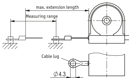
Fig. 2: Extension length check
