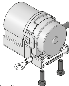
Fig. 1: Mounting
