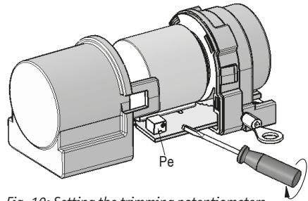
Fig. 10: Setting the trimming potentiometers
