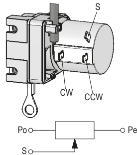
Fig. 5: Potentiometer connection / circuit diagram
