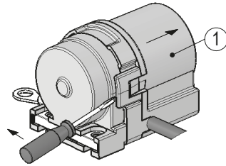
Fig. 4: Opening
